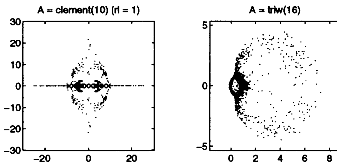
Figure 26.2. Pseudospectra of \text{companion}(A) .
