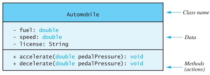
FIGURE 5.2 A Class Outline as a UML Class Diagram
