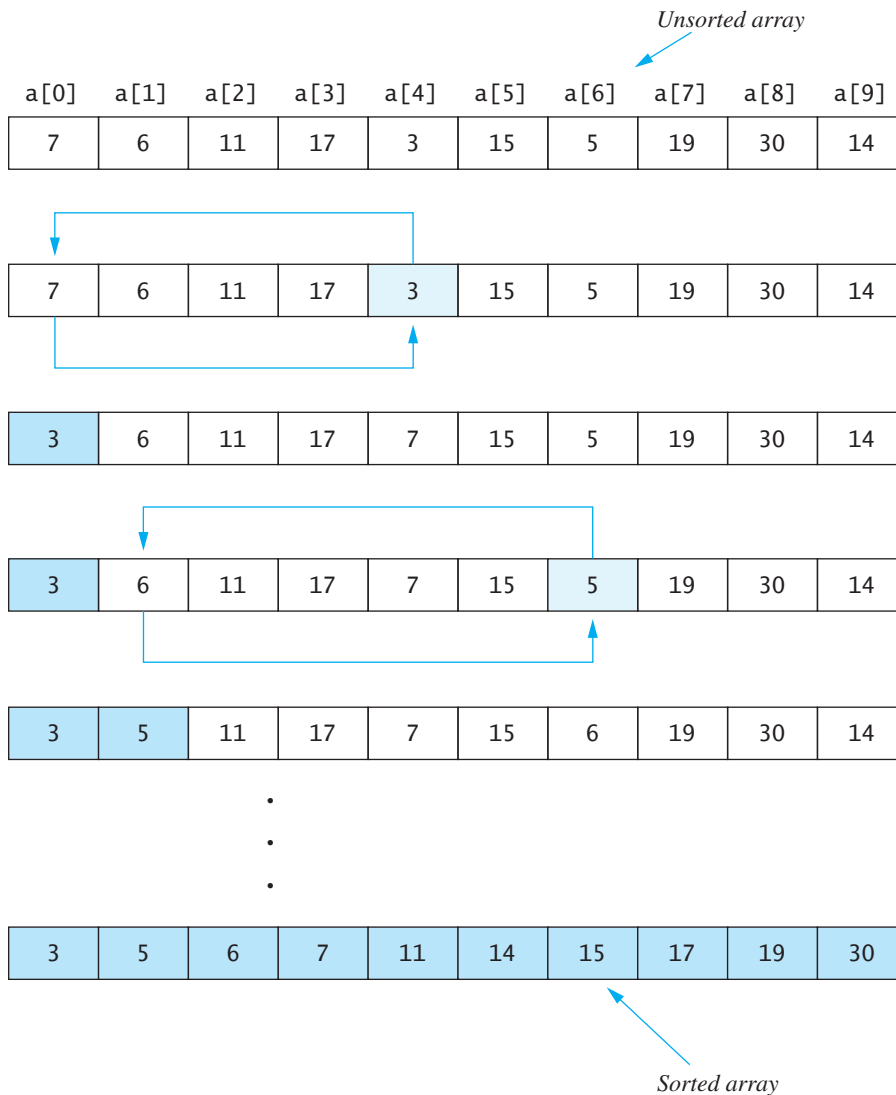
FIGURE 7.5 Selection Sort
