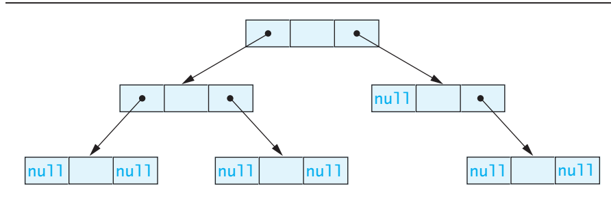
FIGURE 12.12 A Binary Tree
