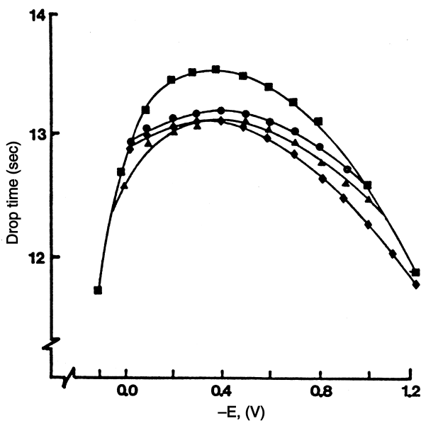
FIGURE 1-16 Electrocapillary curves of background (■), ethynylestradiol (●), \beta -estradiol (▲) and morganstrel (◆). (Reproduced with permission from reference 12.)
