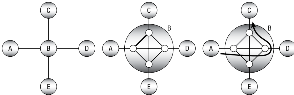
Figure 13.22: You can expand a node to represent turn penalties.
