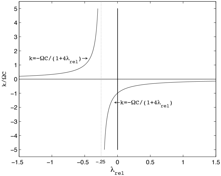
Fig. 3.4 A graph of extremal coordinates k versus Lagrange Multipliers \lambda_{rel}^{\pm} for a fixed spin \Omega > 0 as in equations (3.39) and (3.42).
