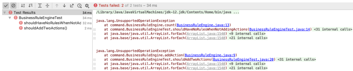
Figure 5-3. Failing tests
