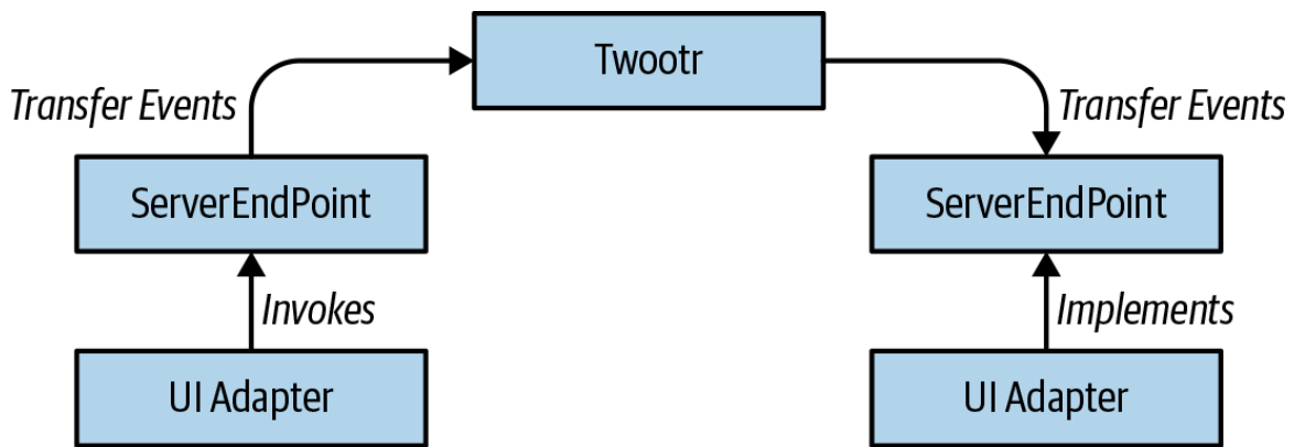
Figure 6-6. Events to code
