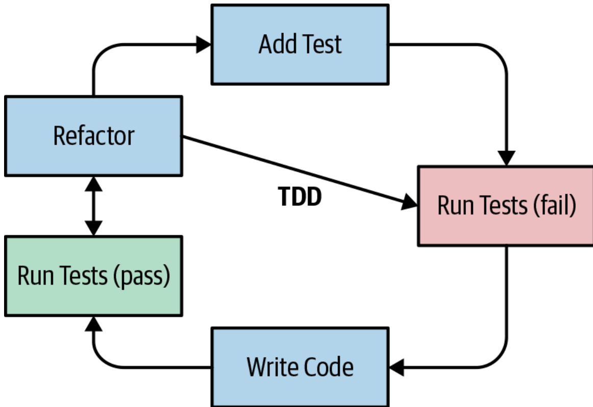
Figure 5-2. TDD with refactoring
