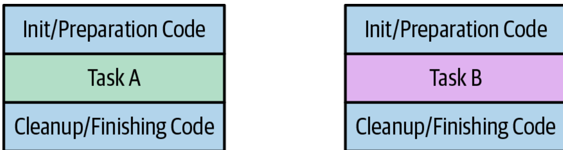
Figure 7-1. Execute Around pattern
