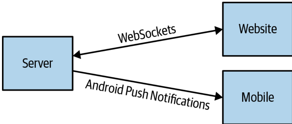
Figure 6-4. Different communications approaches
