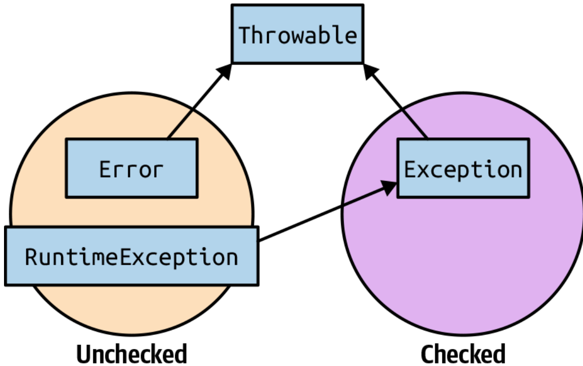
Figure 3-1. Exceptions hierarchy in Java
