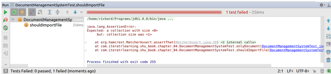
Figure 4-3. Screenshot of assertThat example failing
