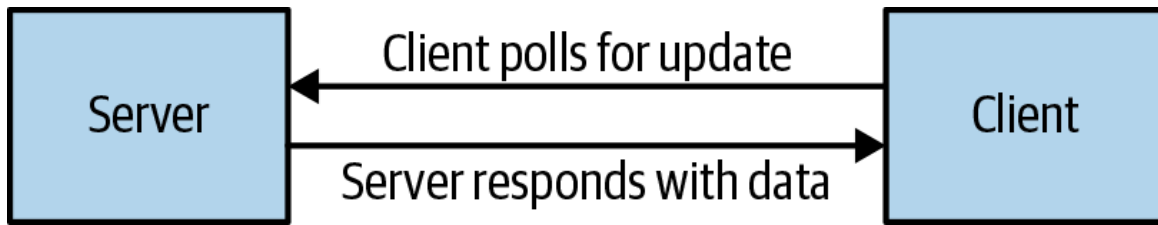
Figure 6-2. Pull communications
