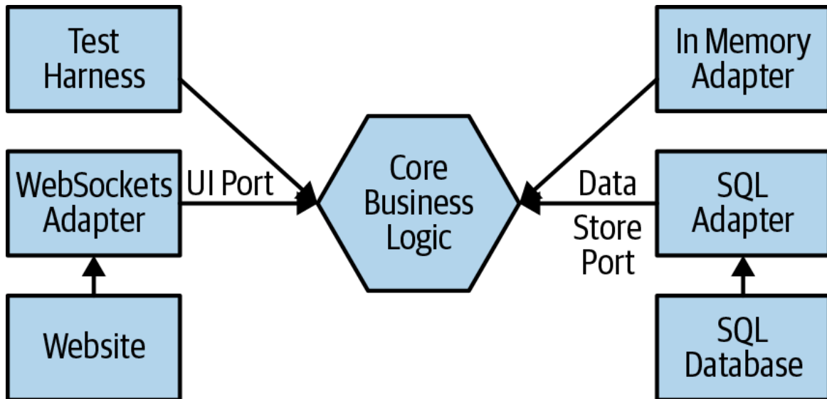
Figure 6-5. Hexagonal architecture
