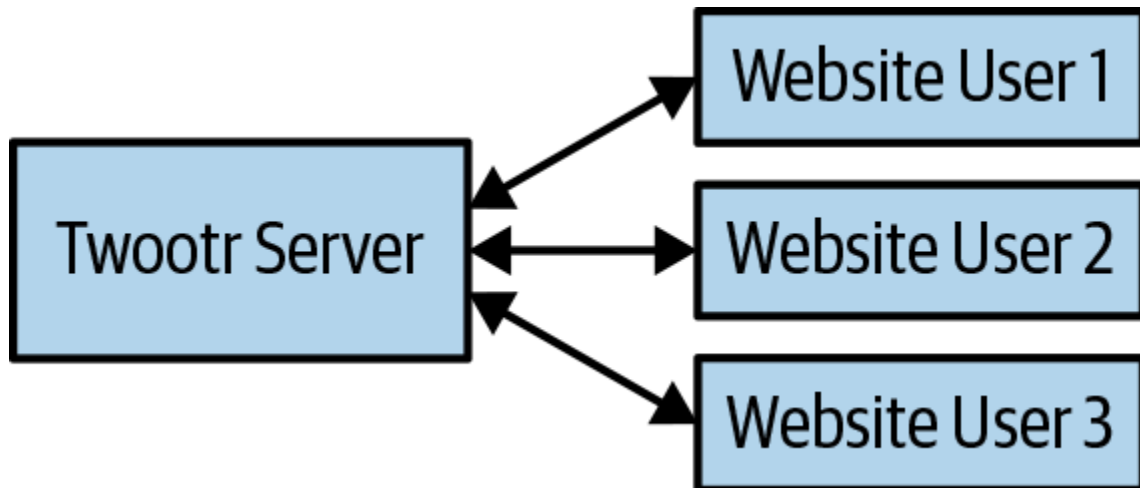
Figure 6-1. Client-server model
