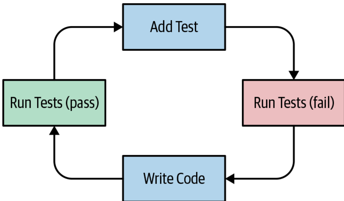
Figure 5-1. TDD cycle
