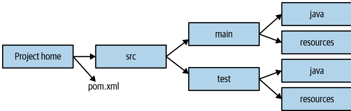
Figure 3-2. Maven standard directory layout
