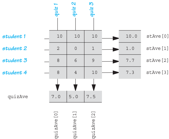
Display 5.12 The Two-Dimensional Array grade
