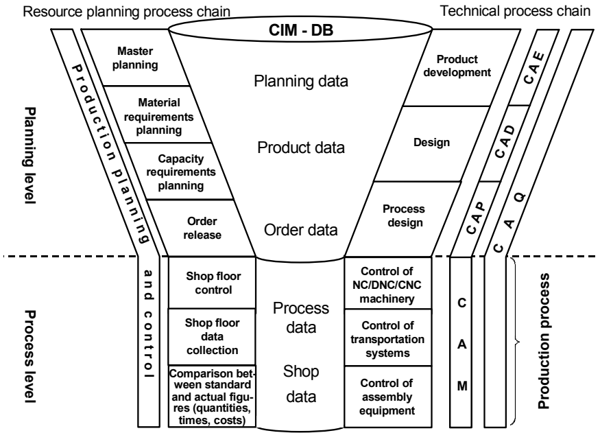
Fig. 16.5.2.3 Integration of order processing functions using a common CIM database.
