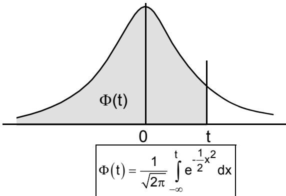
Fig. 10.3.3.5 Normal integral distribution function (service function).
