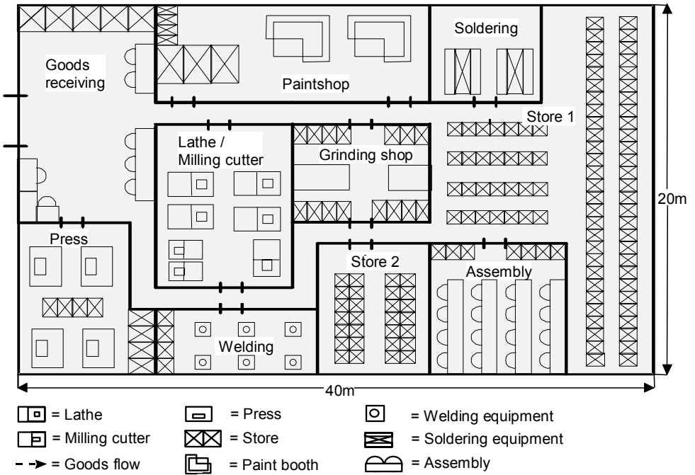
Fig. 3.8.3.1 Company-internal layout with an example process.
