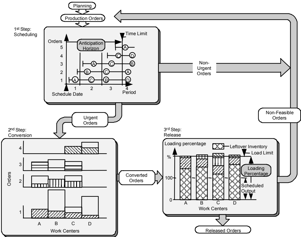
Fig. 14.1.2.2 Steps of load-oriented order release. (From: [Wien95].)
